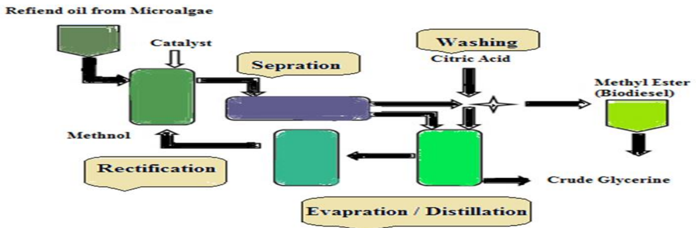
Figure 3: Schematic of esterification process of microalgal oil to biodiesel.
