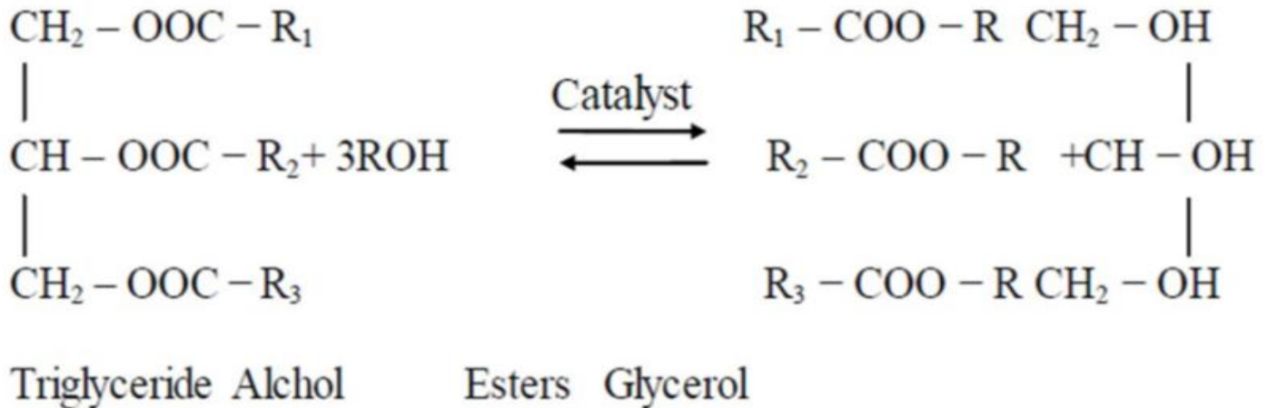
Figure 2: Chemistry of esterification
